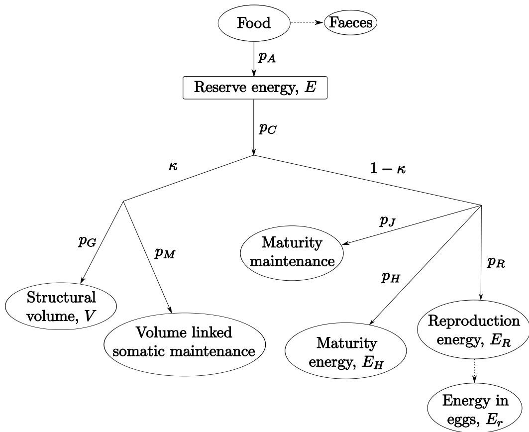
Figure 1. Energy fluxes and the \kappa -rule. It is assumed that a fixed fraction \kappa of utilized energy flows to structural volume and somatic maintenance. See Section 2.1.
