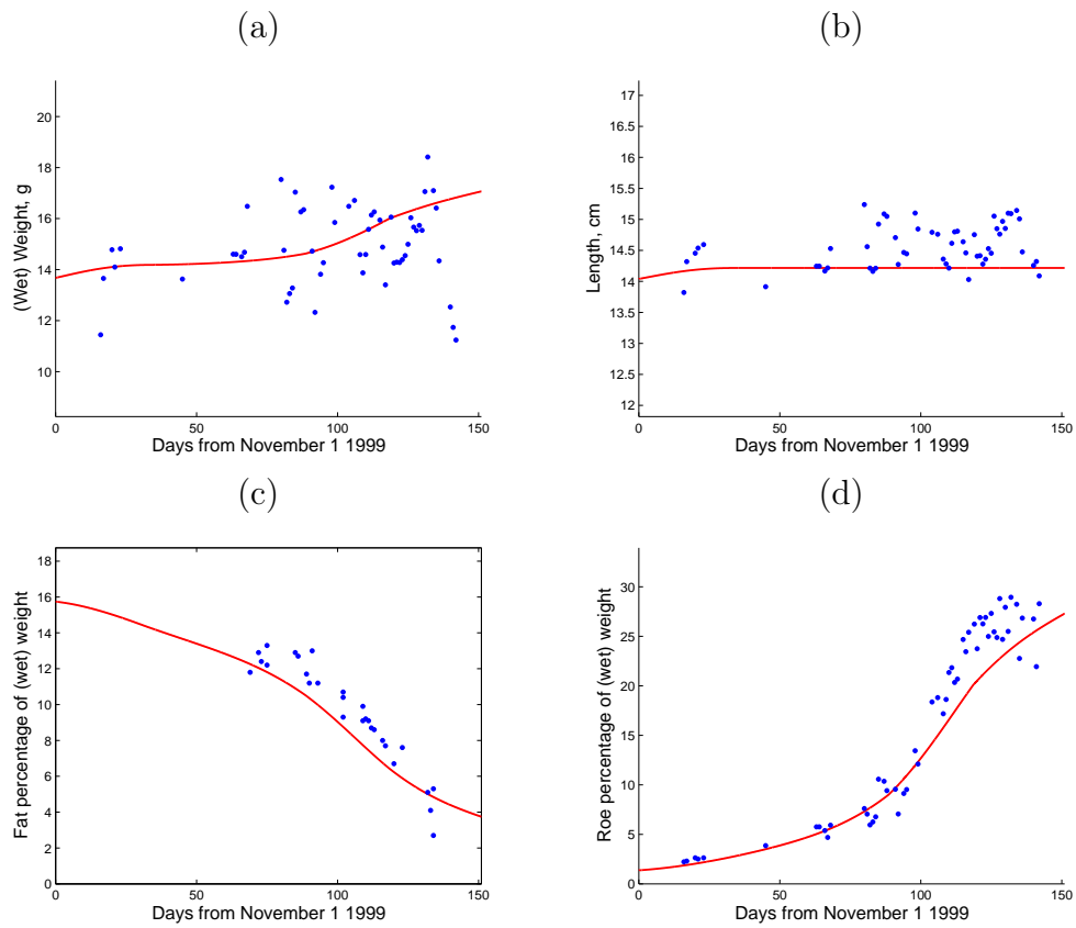
Figure 5. Comparison between measurements of 3 year old mature female capelin during the 1999-2000 season (blue dots) and the DEB model (red curves), see equations (11)-(16). (a) Weight, (b) Length, (c) Fat percentage (d) Roe percentage.
